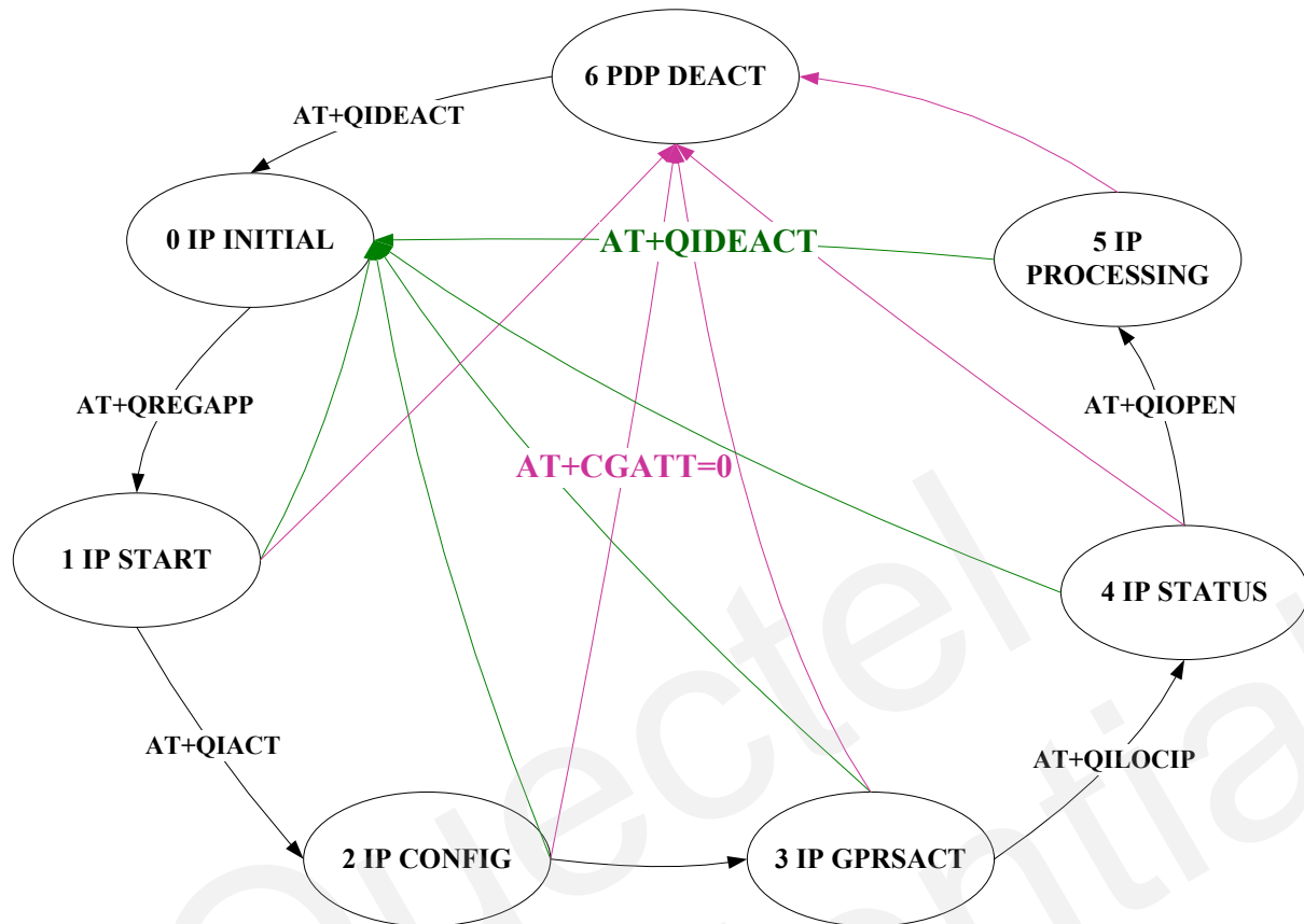
Figure 4: GPRS status of multiple connections
